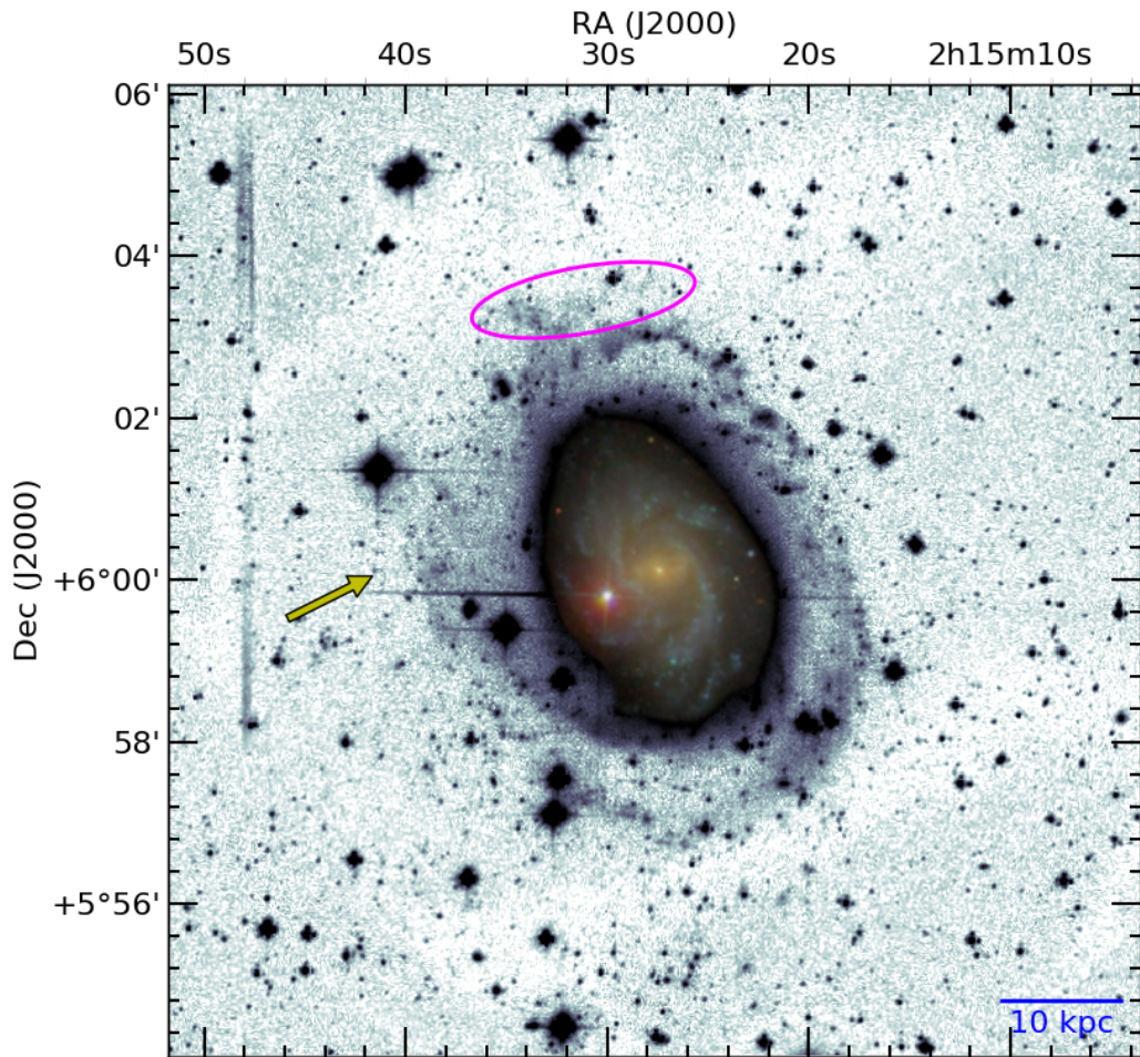
Fig. 3.1 A 12' \times 12' combined image of the Cousins R image from CAHA2.2m telescope and the three photographic B , G , R images from CAHA1.23m telescope. This particular image is only used to show the outer faint structures of the galaxy (e.g. the pseudoring, the Northern region in a magenta ellipse or the Eastern diffuse emission pointed by the yellow arrow), not for any physical measurement. The inner coloured area corresponds to an SDSS image of CIG 96 down to \sim 24 \text{ mag arcsec}^{-2} (SDSS r band) and it is used as reference.
