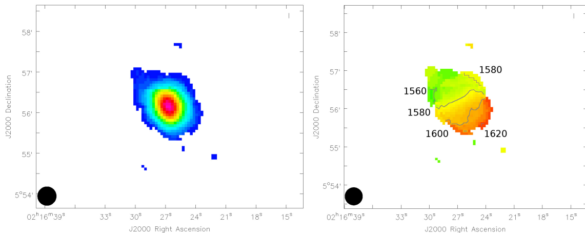
Fig. 4.8 Moment maps of the companion of CIG 96. Left panel : HI integrated intensity map after a 3.5\sigma blanking (see Sect. 3.1.4). Right panel : HI velocity field map after a 3.5\sigma blanking. Grey contours represent the indicated velocities in km s ^{-1} . The black circles at the bottom left of each panel represents the beam size of 28'' \times 28'' .
