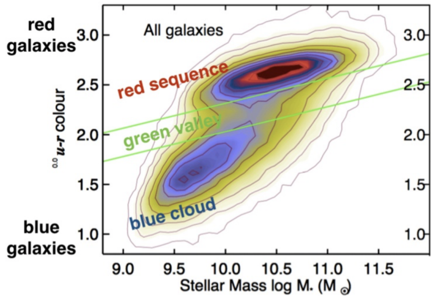
Figure 1.2: Colour-mass diagram for a sample of galaxies observed by SDSS. In the top left, all galaxies are shown, whereas on the right, only early-type (top) and late-type galaxies (bottom) are shown; green lines show the green valley defined by the all-galaxy diagram. The figure is taken from Schawinski et al. (2014) .
