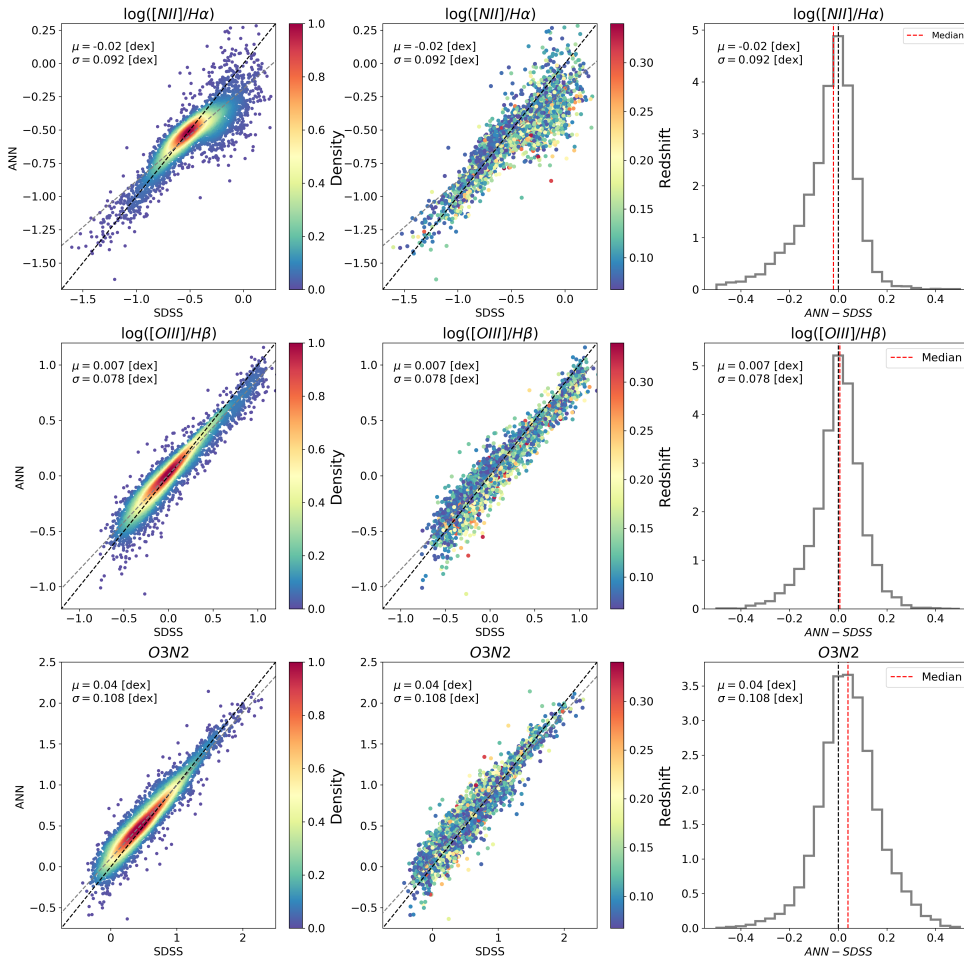
Figure 3.5: Comparison between [N II]/H\alpha , [O III]/H\beta and O3N2 ratios estimated by the ANN_R and SDSS testing sample. Same scheme of Fig. 3.4. The ANN_R is trained with the CALMa set.
