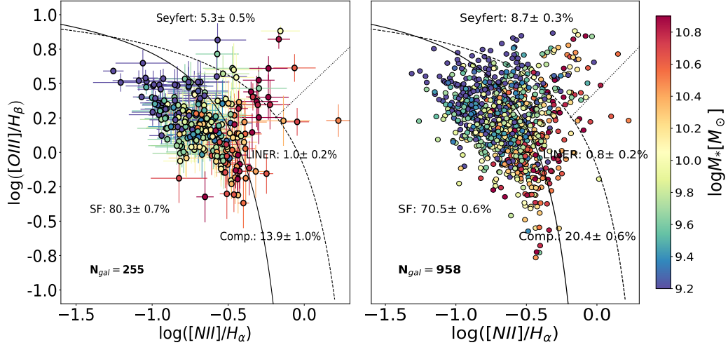
Figure 4.7: BPT diagram for the galaxies in the sample with an error of 0.2 dex (0.5 dex) in the [O III]/H\beta and [N II]/H\alpha ratios in the left (right) panel. The errors are not plotted in the right panel for clarity. The color bar indicates the stellar mass of the galaxy. The solid (Ka03), dashed (Ke01), and dotted lines (S07) define the regions for the four main spectral classes. The relative percentage of each galaxy type in each subsample is indicated in the figure. In each panel, the number of galaxies is specified in the lower left corner. The parent sample contains 2154 galaxies.
