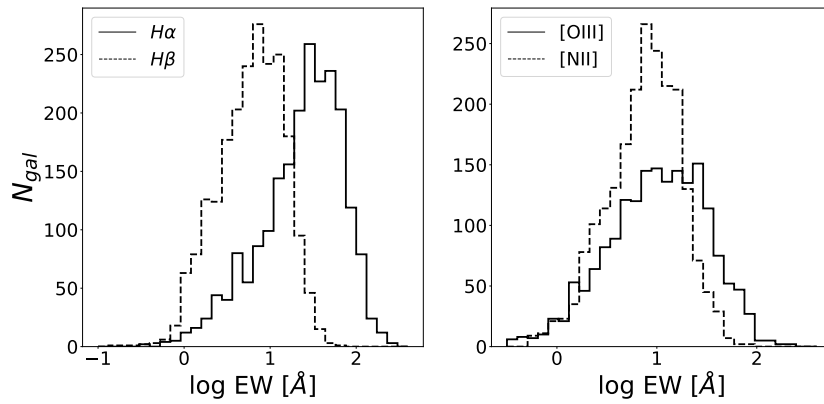
Figure 4.4: Distribution of the EW of H\alpha and H\beta (left), [O III] , and [N II] (right) in log scale as obtained with the ANN_R .
