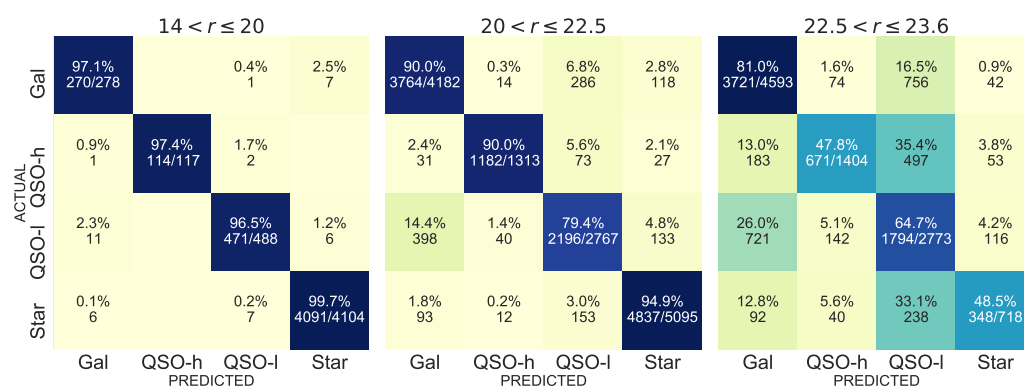
Figure C.3: Confusion matrices obtained with the ANN 2 mix in the test sample.
