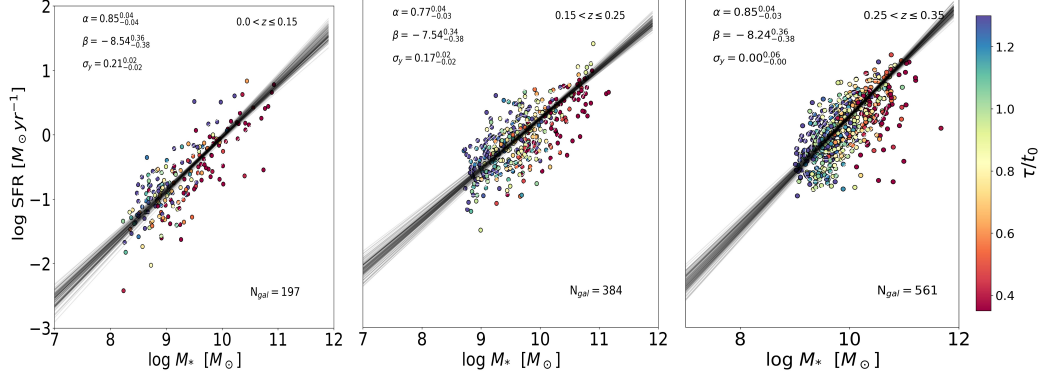
Figure 4.13: SFR vs. stellar mass for galaxies in different redshift bins color-coded with their the \tau/t_0 ratio (see section 4.3.2.) Black lines are the best fits obtained with the Bayesian routine. The median posterior value and 1\sigma confidence interval are shown for each of the parameters. The number of galaxies within each redshift bin is also indicated.
