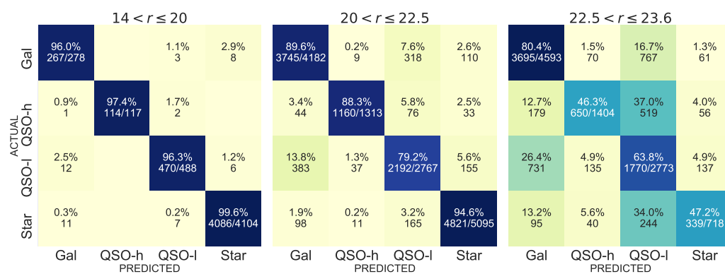
Figure C.2: Confusion matrices obtained with the ANN 2 in the test sample.
