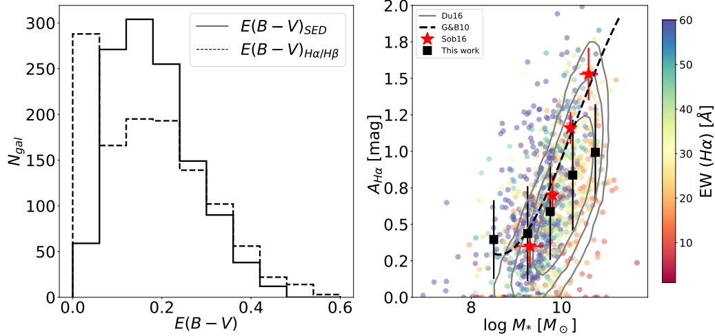
Figure 4.11: Distribution of the nebular ( E(B-V)_{H\alpha/H\beta} ) and stellar ( E(B-V)_{SED} ) color excess (left). Nebular extinction at the H\alpha wavelength as a function of stellar mass (right). Galaxies are color-coded with the EW of H\alpha and belong to the SF sample described in section 4.5.1. Black squares are the median obtained in the following stellar mass bins: 8 < \log M_* \leq 9 , 9 < \log M_* \leq 9.5 , 9.5 < \log M_* \leq 10 , 10 < \log M_* \leq 10.5 , and 10.5 < \log M_* \leq 11 . The error bars on the y-axis represent the standard deviation, gray contours represent the density of sources for 1 \sigma , 2 \sigma , and 3 \sigma derived from SDSS galaxies in Duarte Puertas et al. (2017). Red stars are the values obtained by Sobral et al. (2016) by means of spectroscopy measurements in SF galaxies within the cluster C10939+4713 at z = 0.41 . The dashed black line is the best polynomial fit obtained by Garn & Best (2010) in a sample of SDSS galaxies.
