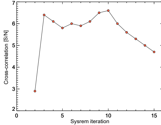
Figure 4.7: Retrieved S/N when cross-correlating the residual matrix after each SYSEM iteration with the \text{H}_2\text{O} absorption model including the p - T profile B and a VMR of 10^{-4} . The values correspond to the highest S/N at the corresponding K_p and v_{\text{wind}} in the range of K_p = 140 to 180 km/s and v_{\text{wind}} = -10 to 10 km/s. The first iteration is not shown for clarity, since it is dominated by telluric residuals.
