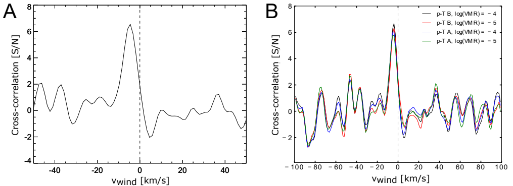
Figure 4.8: A: Total CCF when using the nominal model. The signal is blue-shifted by -3.9 \pm 1.3 km/s. B: CCFs obtained for the studied \text{H}_2\text{O} absorption models. The results are very similar, hence showing a degeneracy in the tested p - T profiles and \text{H}_2\text{O} abundances. A vertical dashed line marks the zero velocity value as a reference in both panels.
