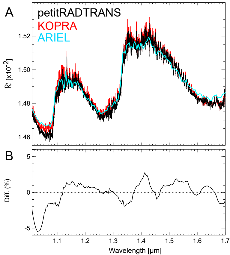
Figure 2.14: Comparison of model transmission spectra during the primary transit of the hot Jupiter HD 209458 b generated with KOPRA (red) and petitRADTRANS (black). The cyan spectrum is that computed by the ARIEL Working Group (see Fig. 2.13) and it is only shown for illustration. The quantity shown in the vertical axis of the top panel is the spectrum ratio, calculated following Eq. 2.49, multiplied by 10^2 . B: Relative differences between the petitRADTRANS and the KOPRA calculations.
