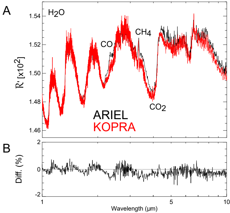
Figure 2.13: A: Comparison of model transmission spectra during the primary transit of the hot Jupiter HD 209458 b generated with KOPRA (red) and those provided by the ARIEL retrieval Working Group (black). The quantity shown in the vertical axis is the spectrum ratio, calculated following Eq. 2.49, multiplied by 10^2 . B: Relative differences between both models.
